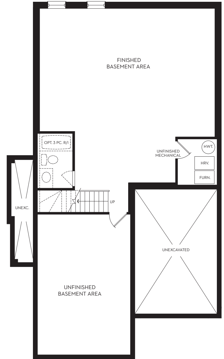
BASEMENT B
